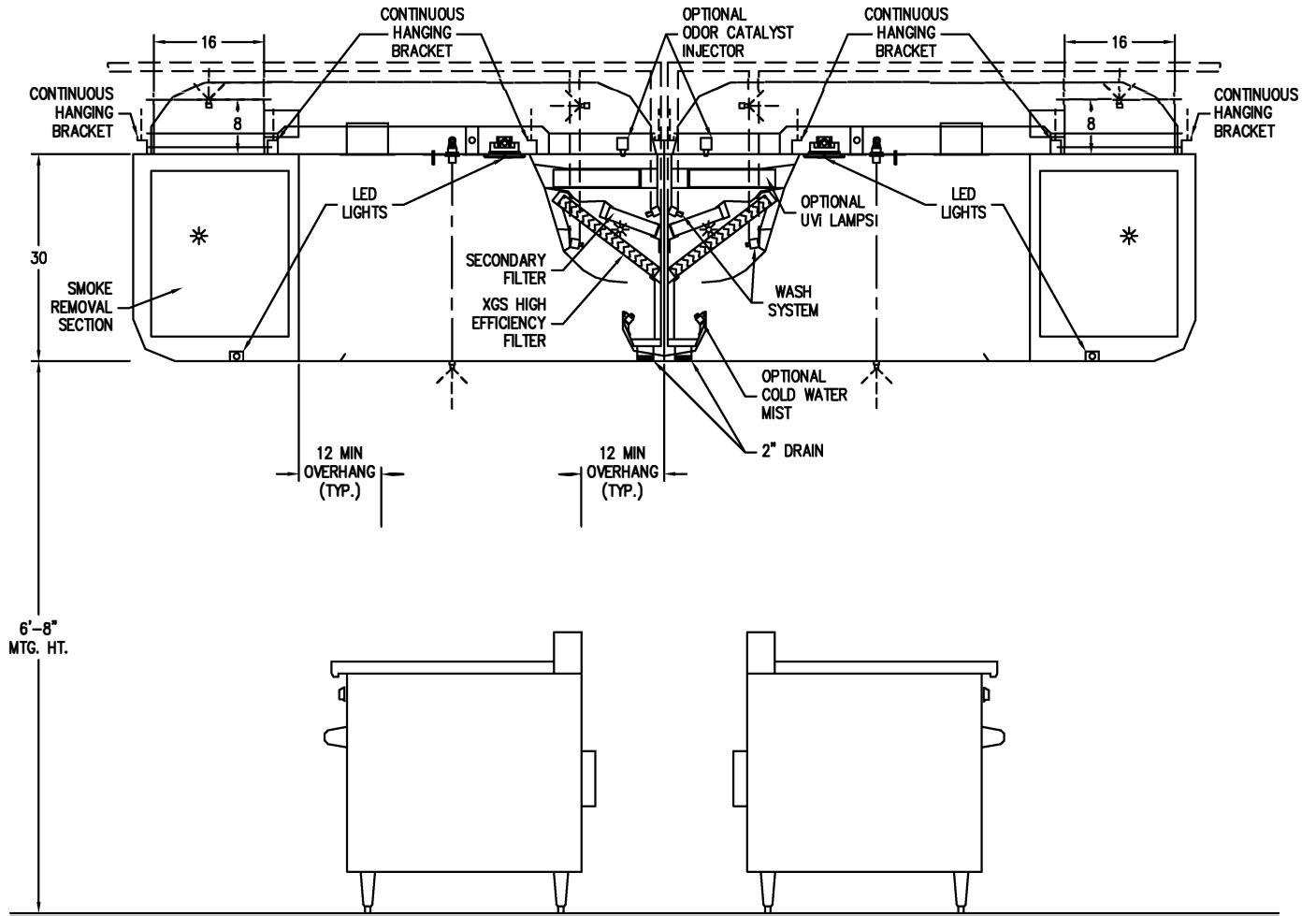
SECTION VIEW
