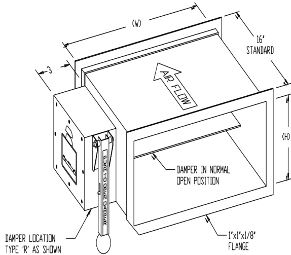
TYPICAL GAYLORD AUXILIARY EXHAUST TERMINAL
