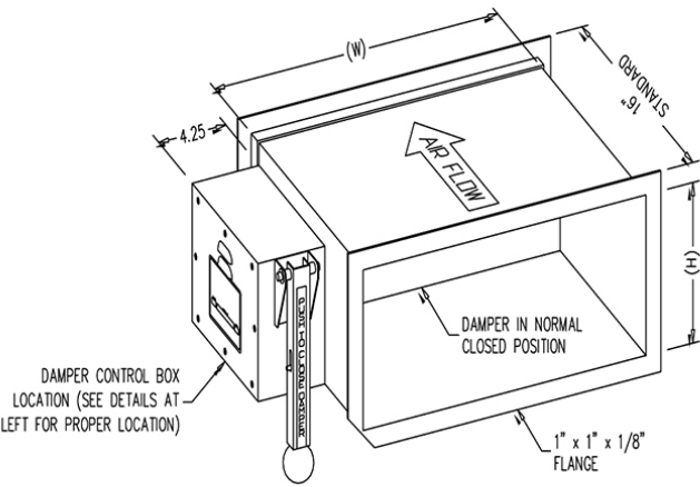
TYPICAL GAYLORD AUXILIARY EXHAUST DE-SMOKE TERMINAL WITH SOLENOID OPERATED DAMPER MODEL: NSD61-(H)-(W)-16-(CONTROL LOCATION)-(MATERIAL)-VOLTAGE
